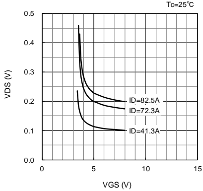
VDS-VGS characteristics (typical)
